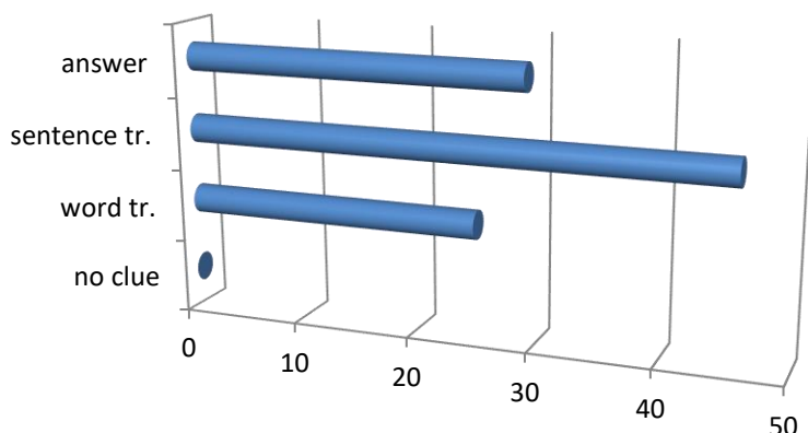
Sentence 4
