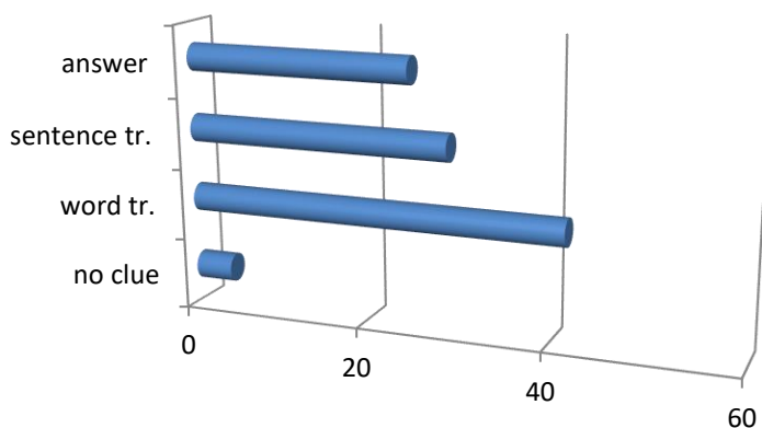
Sentence 7
