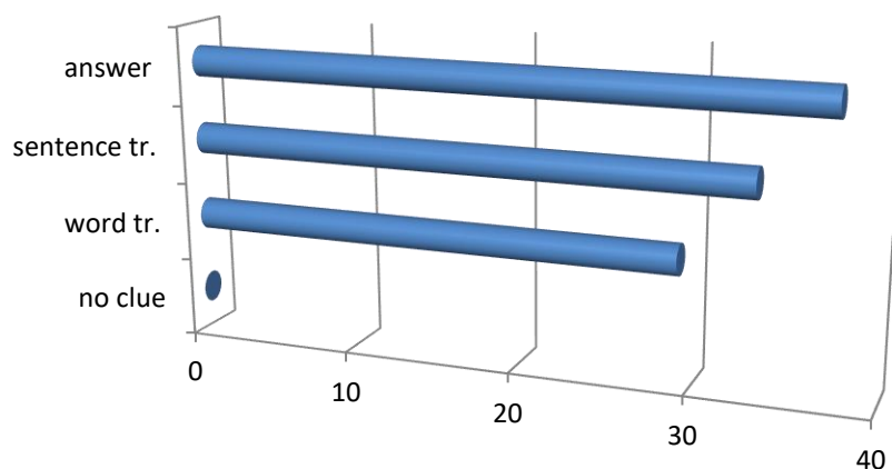
Sentence 9
