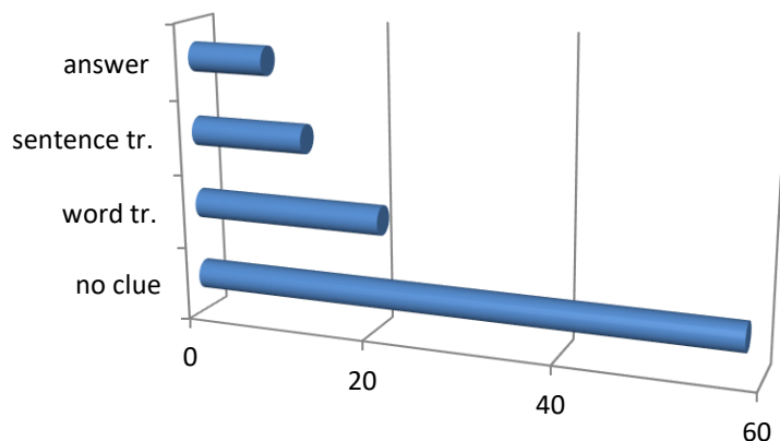
Sentence 8
